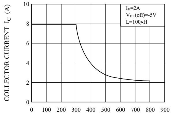
COLLECTOR-EMITTER CLAMP VOLTAGE V_{CE} (V)
